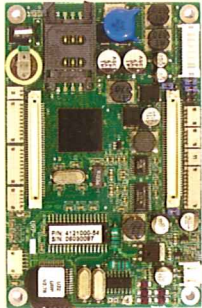
URP Board
