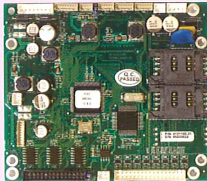
Peripheral Board
