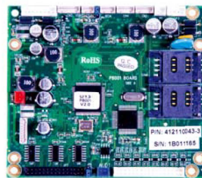
Peripheral board
