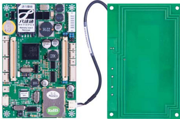
Main board & RF antenna
